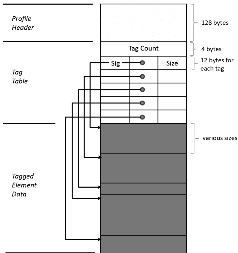
Figure 5 — Profile structure
