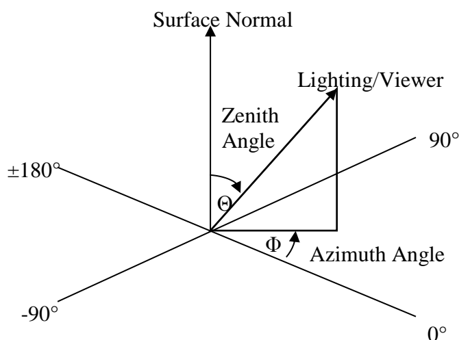
Figure 2 — Normal, zenith and azimuth angles
